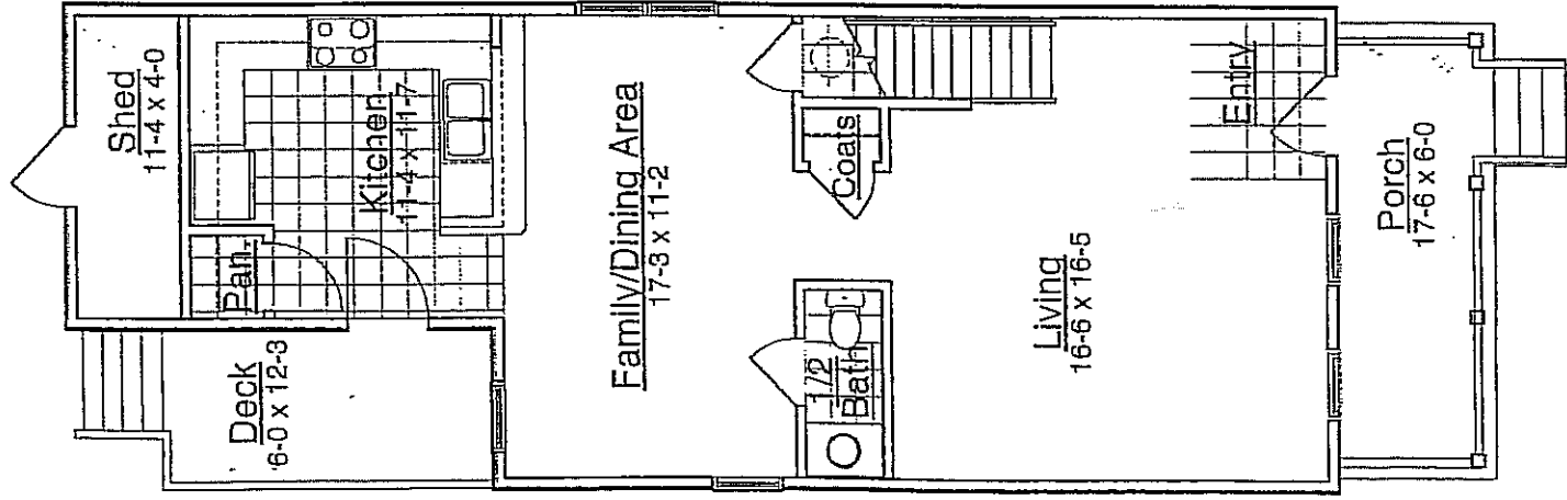
First Floor Plan 1/8" = 1'-0"
